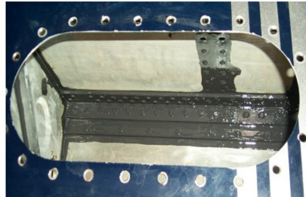
Airplane wing access panel showing applied sealant
